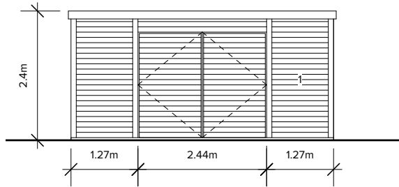
East Elevation (Front)
